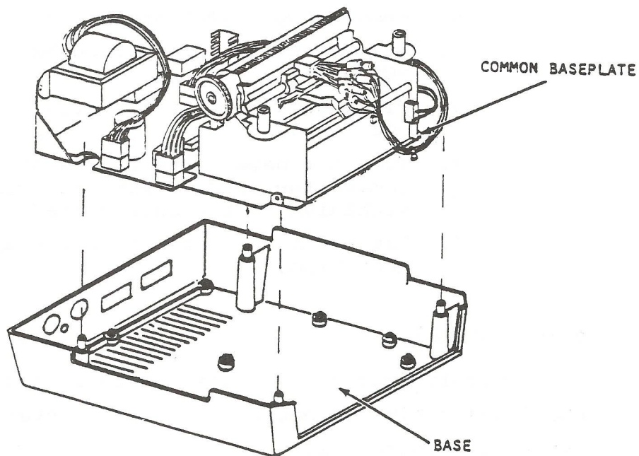
Figure 5-12. Base and Common Baseplate Removal
