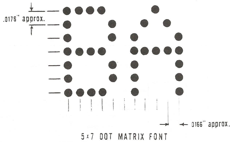
Figure 4-6. Character Font
