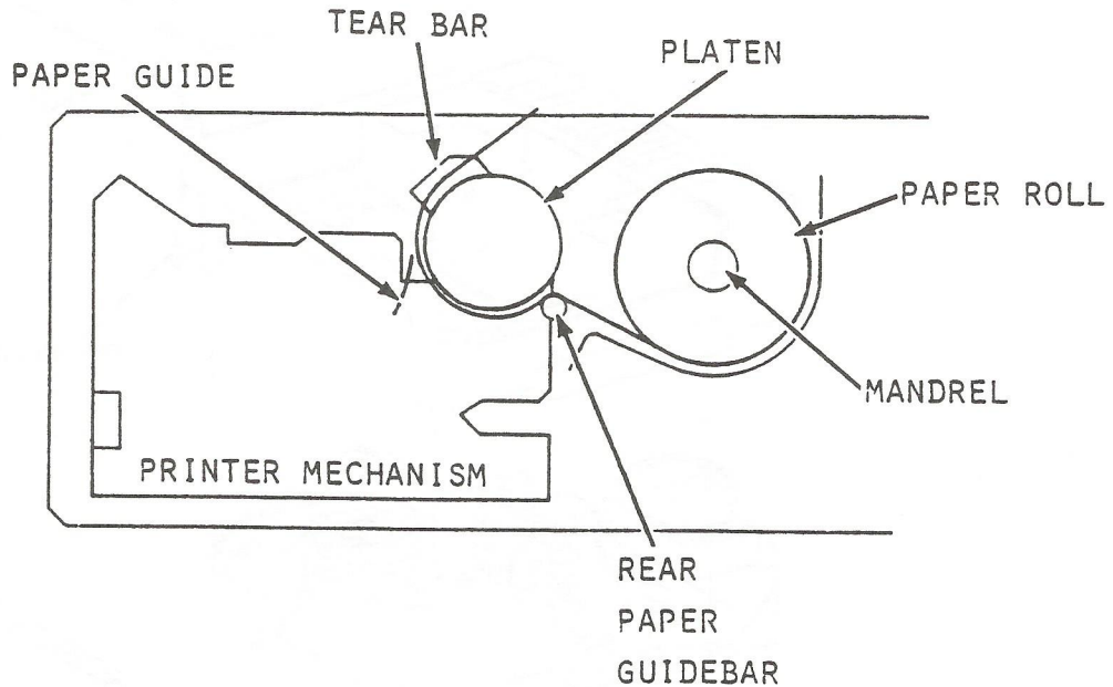
Figure 5-9. Paper Installation Guide
