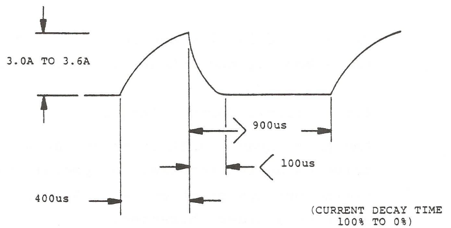
Figure 4-8. Current Waveform
