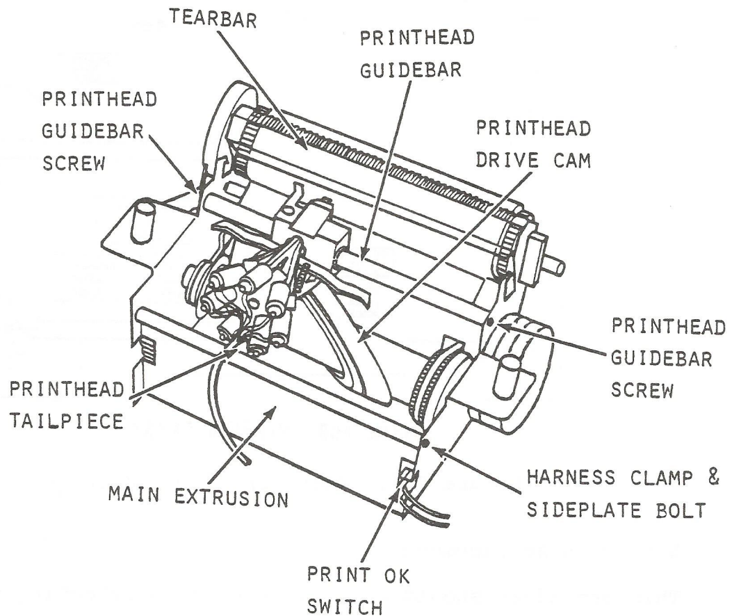
Figure 5-5. Print Mechanism-Component Location
