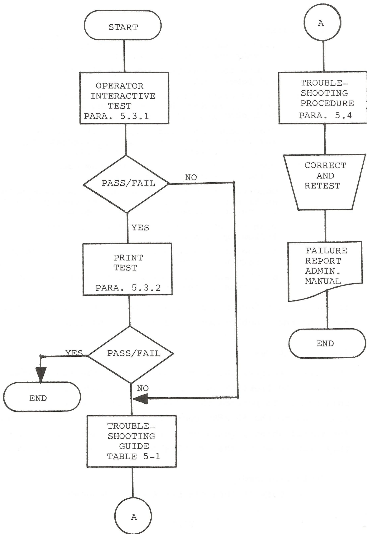
FIGURE 5-1. PRINTER TROUBLESHOOTING FLOWCHART
