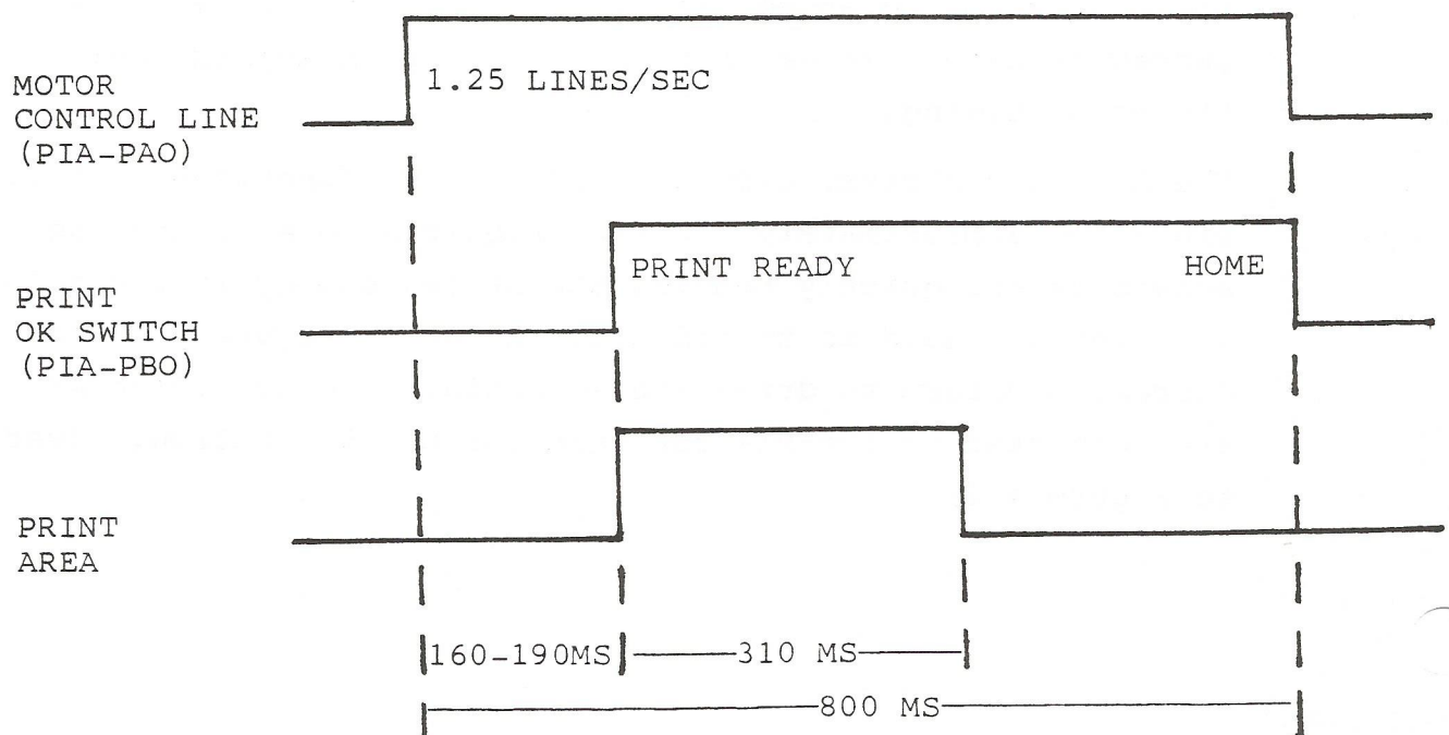
Figure 4-7. Print Timing
