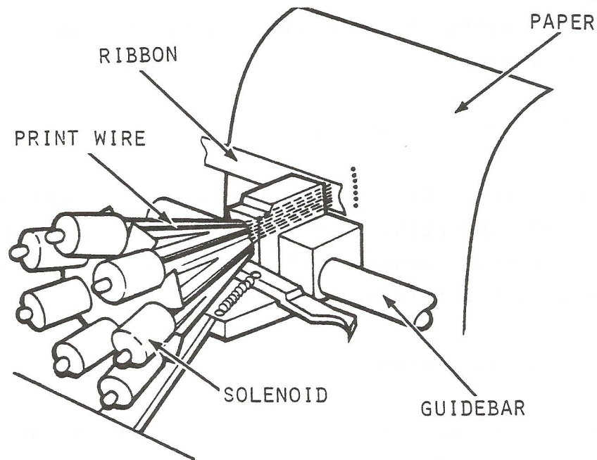
Figure 4-2. Print Head Assembly
